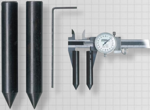
▲ Centerline gages—shown with dial caliper.
